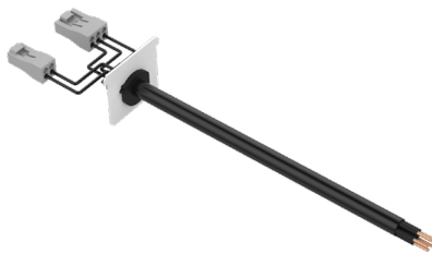
Dry Power Connector with End Cap (A1-ZAFU-STN-PC-EC-Y-DRY-X) Y = Lens / Optics X = Specify Cable Length, 6' Default
