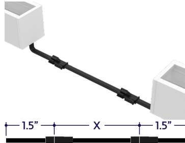
Dry Continuous Connector with Black Jacket (A1-ZAKY-SSQ-CC-BFF-DRY-BK-X) X = Specify Length, 3" Default
