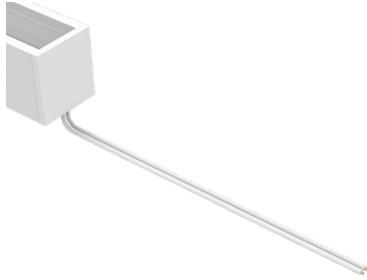
Dry Power Connector (A1-ZAKY-SSQ-PC-BFF-DRY-X) X = Specify Length, 36" Default, 25' Maximum
