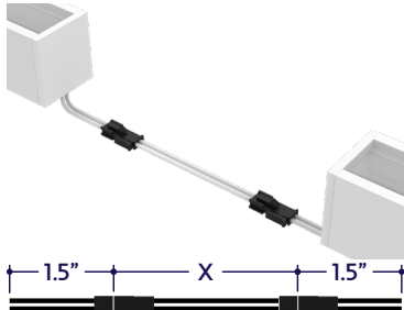
Dry Continuous Connector (A1-ZAKY-SSQ-CC-BFF-DRY-X) X = Specify Length, 3" Default
