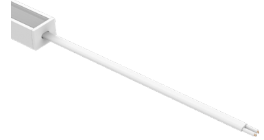
Dry Power Connector with White Jacket (A1-ZAKY-STN-PC-DRY-WH-X) X = Specify Length, 36" Default, 25' Maximum
