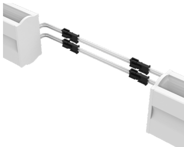
Dry Continuous Connector (A1-ZAKY-SWD-CC-BFF-DRY-X) X = Specify Length, 3" Default
