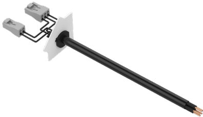
Dry Power Connector with Left End Cap (A1-ZENU-SNK-PC-ECL-Y-DRY-X) Y = Lens / Optics X = Specify Cable Length, 6' Default
