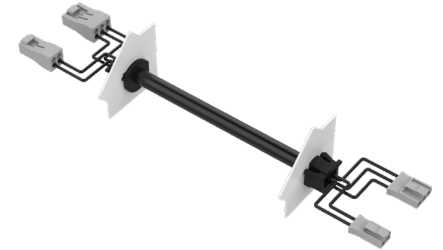
Dry Jumper Cable with End Caps (A1-ZENU-SNK-JC-EC-Y-DRY-X) Y = Lens / Optics X = Specify Cable Length, 6' Default
