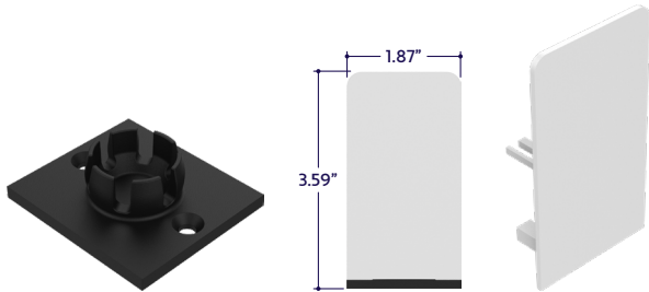
Dry Location End Cap (A1-ZYZY-SQR-EC)
