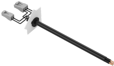
Dry Power Connector with Left End Cap (A1-ZENU-STN-PC-ECL-Y-DRY-X) Y = Lens / Optics X = Specify Cable Length, 6' Default
