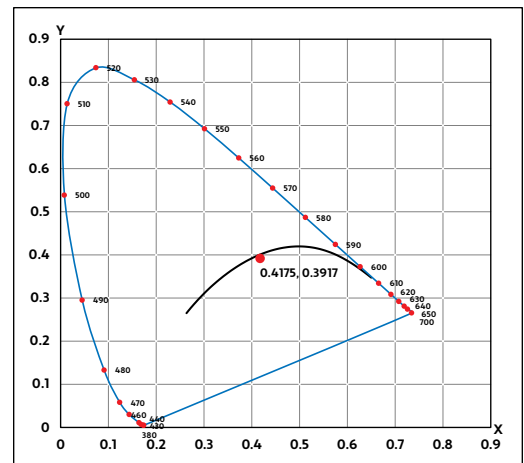
Chromaticity Diagram
