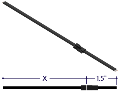
Dry Power Connector with Black Jacket 20/2 Gauge Wire (A8-PC-2P-DRY-BK-X) X = Specify Length, 36" Default
