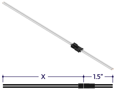
Dry Power Connector 20/2 Gauge Wire (A8-PC-2P-DRY-X) X = Specify Length, 36" Default
