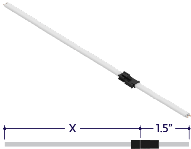
Dry Power Connector with White Jacket 20/2 Gauge Wire (A8-PC-2P-DRY-WH-X) X = Specify Length, 36" Default
