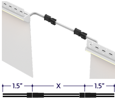
Dry Continuous Connector (20/2 Gauge Wire) (A8-ZIGY-FPA-CC-SFF-DRY-X) X = Specify Length, 3" Default
