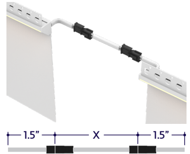
Dry Continuous Connector with White Jacket (20/2 Gauge Wire) (A8-ZIGY-FPA-CC-SFF-DRY-WH-X) X = Specify Length, 3" Default
