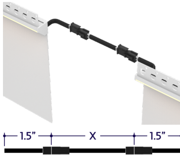
Dry Continuous Connector with Black Jacket (20/2 Gauge Wire) (A8-ZIGY-FPA-CC-SFF-DRY-BK-X) X = Specify Length, 3" Default
