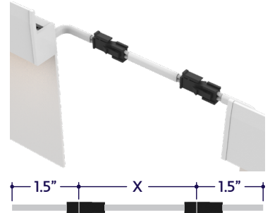
Dry Continuous Connector with White Jacket (20/2 Gauge Wire) (A8-ZIGY-RPB-CC-SFF-DRY-WH-X) X = Specify Length, 3" Default
