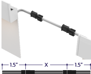
Dry Continuous Connector (20/2 Gauge Wire) (A8-ZIGY-RPB-CC-SFF-DRY-X) X = Specify Length, 3" Default
