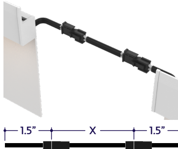
Dry Continuous Connector with Black Jacket (20/2 Gauge Wire) (A8-ZIGY-RPB-CC-SFF-DRY-BK-X) X = Specify Length, 3" Default
