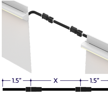
Dry Continuous Connector with Black Jacket (20/2 Gauge Wire) (A8-ZIGY-SPA-CC-SFF-DRY-BK-X) X = Specify Length, 3" Default
