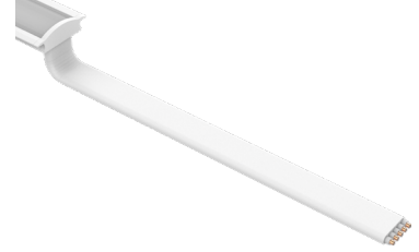
Dry Power Connector with White Jacket (20/5 Gauge Wire) (A8-ZIZA-RCL-PC-BFF-DRY-WH-X) X = Specify Length, 36" Default, 25' Maximum
