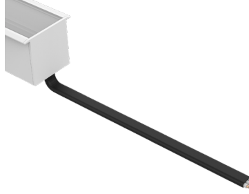
Dry Power Connector with Black Jacket (20/3 Gauge Wire) (A8-ZOMU-RCD-PC-BFF-DRY-BK-X) X = Specify Length, 36" Default, 25' Maximum
