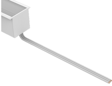
Dry Power Connector (20/3 Gauge Wire) (A8-ZOMU-RCD-PC-BFF-DRY-X) X = Specify Length, 36" Default, 25' Maximum
