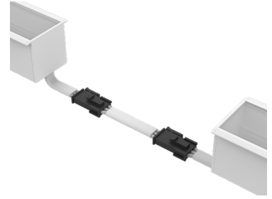
Dry Continuous Connector with White Jacket (20/3 Gauge Wire) (A8-ZOMU-RCD-CC-BFF-DRY-WH-X) X = Specify Length, 3" Default
