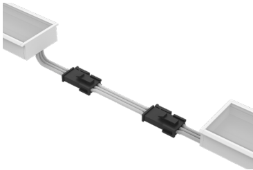
Dry Continuous Connector (20/3 Gauge Wire) (A8-ZOMU-RCL-CC-BFF-DRY-X) X = Specify Length, 3" Default
