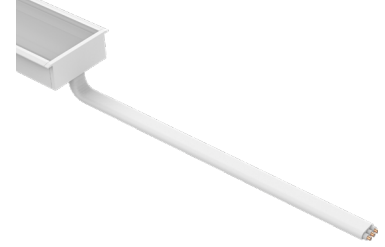
Dry Power Connector with White Jacket (20/3 Gauge Wire) (A8-ZOMU-RCL-PC-BFF-DRY-WH-X) X = Specify Length, 36" Default, 25' Maximum
