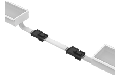
Dry Continuous Connector with White Jacket (20/3 Gauge Wire) (A8-ZOMU-RCL-CC-BFF-DRY-WH-X) X = Specify Length, 3" Default
