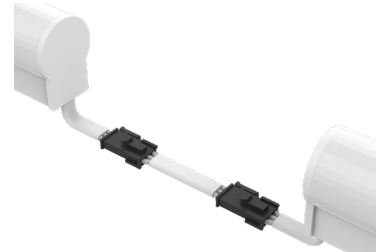
Dry Continuous Connector with White Jacket (20/3 Gauge Wire) (A8-ZUDA-SSR-CC-BFF-DRY-WH-X) X = Specify Length, 3" Default
